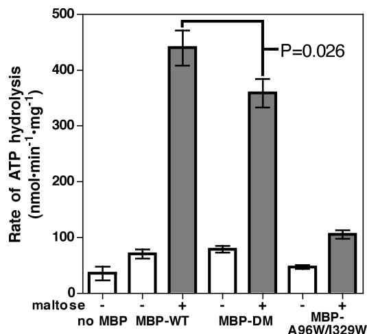
FIGURE 8: Destabilization of the open conformation decreases MalFGK 2 ATPase. The ability of wild-type MBP (MBP-WT), MBP-DM, and MBP-A96W/I329W to stimulate the MalFGK 2 ATPase was measured in either the absence (hollow bars) or presence (filled bars) of 5 mM maltose. An MBP concentration of 2 \mu M was used in each case, and measurements were made in triplicate; the mean value is shown with error bars representing the standard deviation. The PLS on their own (hollow bar, far left) show a low basal ATPase that is doubled by the addition of unliganded MBP and increased over 10-fold by the addition of MBP and maltose. In the presence of maltose, MBP-DM does not stimulate the MalFGK 2 ATPase to the same degree as wild-type MBP. MBP-A96W/I329W shows a severely impaired ability to stimulate MalFGK 2 in both the absence and presence of maltose.
