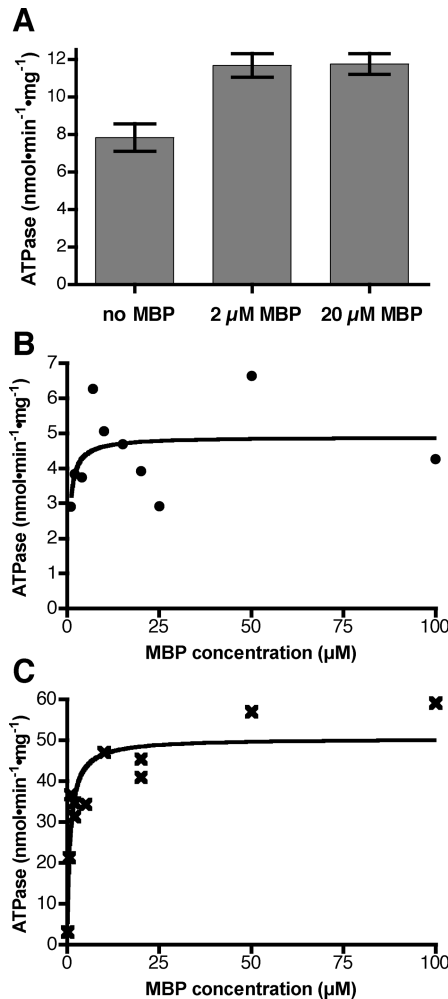
FIGURE 3: Kinetic analysis of MBP-MalFGK 2 ATPase stimulation in the absence of maltose. (A) In the absence of maltose, MBP produces a small but significant stimulation of the MalFGK 2 ATPase that is exactly the same for 2 μM and 20 μM concentrations of MBP at 20 °C. The bars show the mean ± SD for 6 to 9 determinations in each case. (B) At 20 °C and in the absence of maltose, increases in MBP concentration from 1 to 100 μM produced no significant increase in MalFGK 2 ATPase activity (●). Note that activities below 1 μM MBP concentration could not be reliably determined at 20 °C. (C) At 37 °C and in the absence of maltose, the higher activity levels allowed the measurement of the MalFGK 2 ATPase activity at MBP concentrations below 1 μM (×). The data in panels B and C yielded K_M values of less than 1 μM and V_{MAX} values of 5 and 50 nmol·min -1 ·mg -1 at 20° and 37°, respectively. For the analysis in panels B and C, the basal ATPase of the proteoliposomes (in the absence of any MBP) was subtracted from all measurements.
