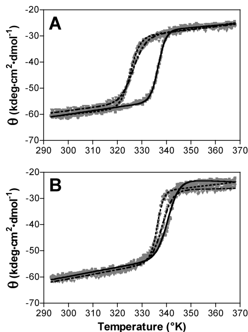
FIGURE 7: Stability of conformationally engineered MBP molecules. Conformationally engineered MBP molecules, MBP-DM and MBP-A96W/I329W, were produced by making changes in the balancing interface that controls opening and closing of the maltose binding cleft (20, 21). The thermal stabilities of MBP-DM (short dashes) and MBP-A96W/I329W (long/short dashes) were compared to wild-type MBP (solid) in the (A) absence of maltose and (B) presence of 500 μM maltose. The samples were heated at 75 K per h, and mean residue ellipticity ( \theta ) at 222 nm was measured every 4 s (gray data points; squares for wild-type MBP, circles for MBP-DM, and inverted triangles for MBP-A96W/I329W). The curves are nonlinear least-squares fits of the data to an equation describing thermodynamic transitions in terms of the two plateau regions (see Materials and Methods). The balancing interface mutations have decreased the stability of the unliganded conformation, but have no significant effect on the stability of the maltose-bound closed conformation.
