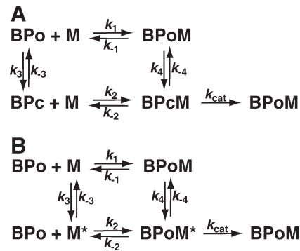
FIGURE 4: Kinetic models for stimulation of MalFGK 2 ATPase by open and closed MBP. (A) Stimulation by closed MBP. Both open and closed forms of MBP (BPO and BPc, respectively) interact with MalFGK 2 , but only the closed form stimulates ATP hydrolysis. In this model, the mechanism of ATPase stimulation is the same for both unliganded and liganded MBP: the closed conformation interacts with MalFGK 2 leading to ATP hydrolysis. In the absence of maltose, the relatively low rate of ATP hydrolysis is due to the limiting concentration of closed, unliganded MBP. (B) Stimulation by open MBP. The stimulation is due to a second conformation of MalFGK 2 (M*) that is separated from its more predominant resting or ground state (M) by an energetic barrier. Open unliganded MBP binds with high affinity to this form of MalFGK 2 , which leads directly to the formation of the transition state for ATP hydrolysis. In this system, the low rate of ATP hydrolysis in the absence of maltose is due to the slow rate of conversion between M and M*. Relative values for the rate constants are provided in Table 2.
