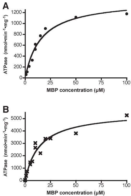
FIGURE 2: Kinetic analysis of MBP-MalFGK 2 ATPase stimulation in the presence of maltose. The ability of wild-type MBP to stimulate the MalFGK 2 ATPase, at MBP concentrations from 2 to 100 \mu M, was measured in the presence of 5 mM maltose at (A) 20 °C (●) and (B) 37 °C (×). The solid curves show the nonlinear least-squares fits to the Michaelis–Menten equation, which yielded K M values (defined as the concentration of MBP that yields half maximal ATPase) of approximately 15 \mu M and V MAX values of 1400 and 5500 nmol·min -1 ·mg -1 at 20° and 37°, respectively (Table 1). Note that all MBP preparations included an unfolding and refolding step, as described in Materials and Methods, to completely remove the ligand.
