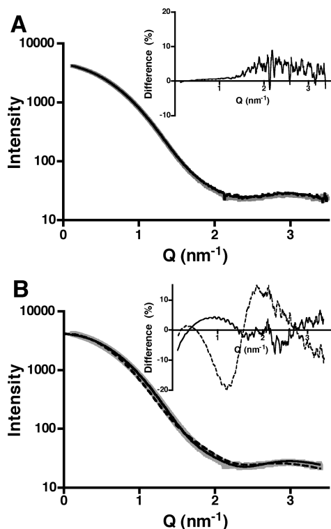
FIGURE 6: Unliganded MBP-A96W/I329W is in a closed conformation. (A) Small-angle X-ray scattering (SAXS) from MBP-A96W/I329W was measured in the absence (thick gray curve) and presence (thin black curve) of maltose. The inset graph shows the difference between the two curves, expressed as a percentage of the total signal. The two curves are almost identical, indicating no observable effect of maltose on the solution conformation of the protein. (B) The SAXS data from unliganded MBP-A96W/I329W (thick gray curve) was matched to the open structure of MBP (PDB ID 1OMP (43) dashed curve) and the closed, ligand-bound structure (PDB ID 1ANF (44) solid curve). The inset shows the difference between the models and the solution conformation of unliganded MBP-A96W/I329W as a percentage of the total signal. The closed conformation of MBP is a better model for the solution conformation of unliganded MBP-A96W/I329W.
