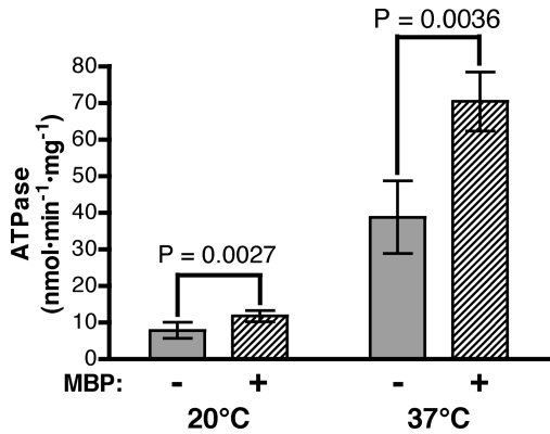
FIGURE 1: Stimulation of the MalFGK 2 ATPase by unliganded MBP. ATP hydrolysis was measured for proteoliposomes on their own (solid gray bars) as well as with 2 \mu M MBP (stippled bars) at 20° and 37°. The addition of MBP resulted in a 50% increase in ATPase activity at 20° and a 100% increase at 37°. Shown are the mean \pm S. D.; a paired t -test was used to calculate the likelihood that the differences arose by chance.
