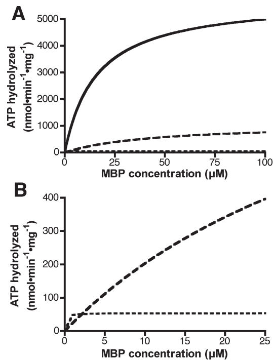
FIGURE 5: Expected rate curves for MalFGK 2 stimulation by MBP. The kinetic models in Figure 4 along with rate constants in Table 2 were used to derive curves for the rate of ATP hydrolysis as a function of MBP concentration. Panels A and B represent the same graphs, but with expanded axes in panel B. In the presence of saturating maltose (solid curve), where all the binding protein is in a closed conformation (accomplished in the model by making the closed to open rate constants very small), the system shows a K_M for MBP of 15 \mu\text{M} , corresponding to what was observed experimentally. In the absence of maltose, the model where the closed, unliganded form is responsible for the stimulation leads to a K_M of just over 40 \mu\text{M} (long dashes) and a significant increase in activity as the concentration of MBP is raised in the region from 1 to 25 \mu\text{M} . Activation by open unliganded MBP (short dashes), as illustrated in Figure 4B and outlined in the text, yields results that are similar to what is observed experimentally.
